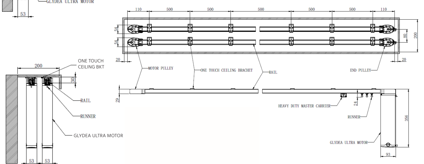
Glydea ULTRA Dimensions - DOUBLE Track
