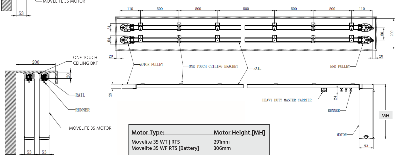
Glydea Track Dimensions - DOUBLE Track
