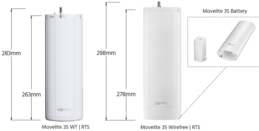
Movelite 35 WT | RTS Motor 240V AC
