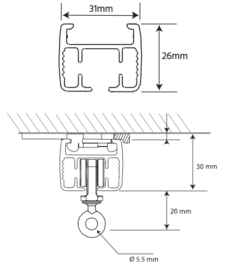
Glydea Curtain Track
