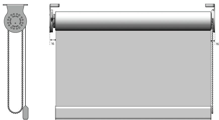
Ambience Heavy Duty Roller Blind System
