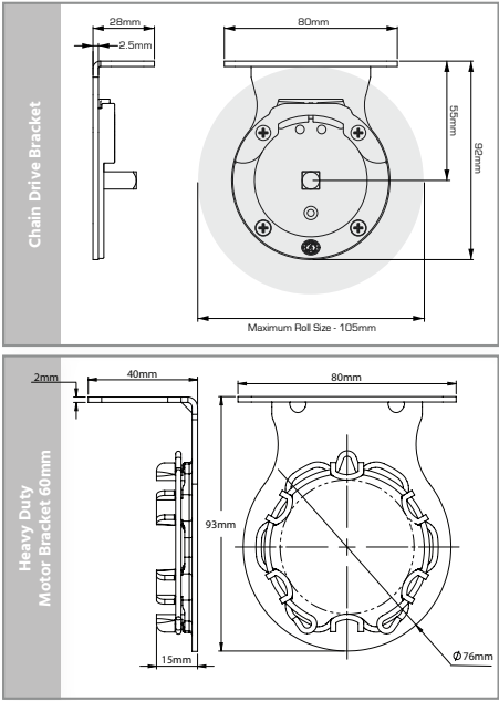
Chain Drive | Motor Bracket | 60mm - 80mm
