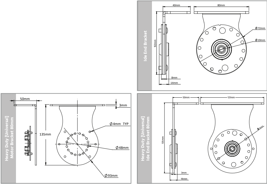
Idle End Bracket
